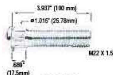
9709-R
