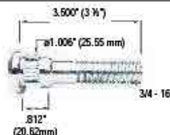
5101A-R
