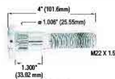
9729-R
