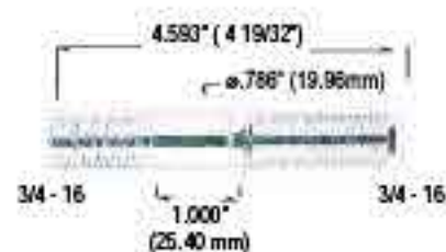
8140N-R / 8141N-L
